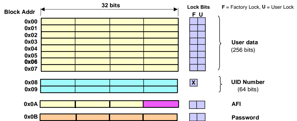
Figure 2 Memory organization of the Tag-it HF-I Pro Transponder IC
