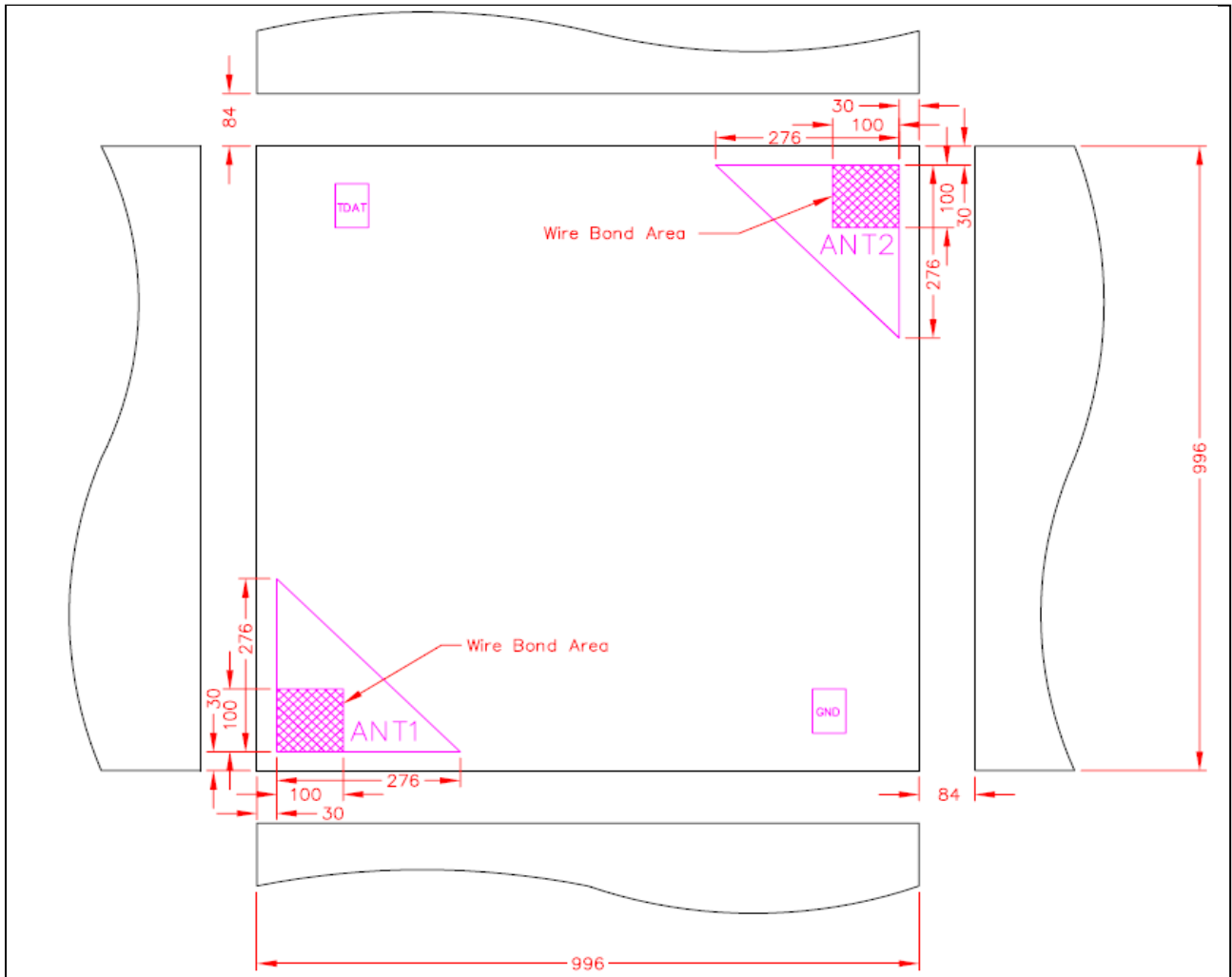
Figure 4 Antenna and Test Pad Location
