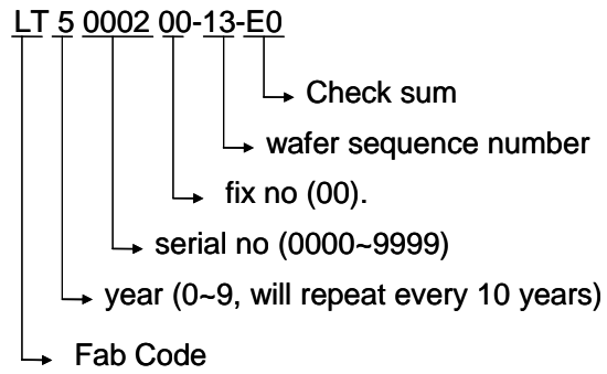
Figure 7 Waferidentification Code 1
